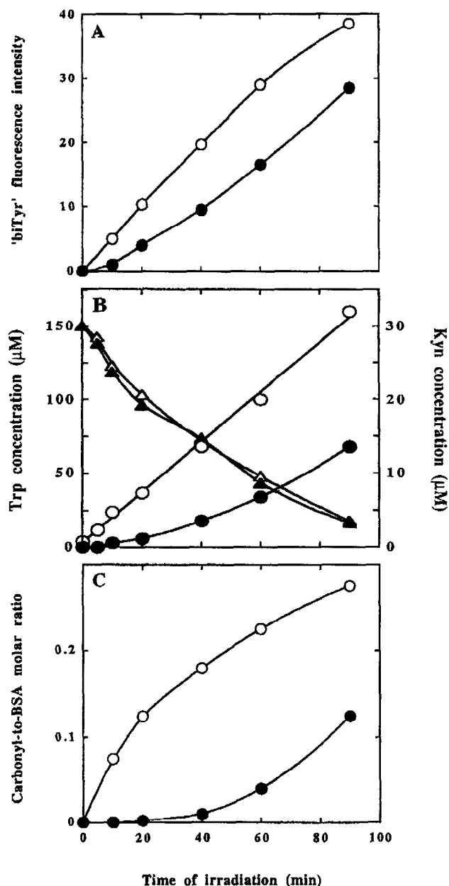
Fig. 2. \gamma -Irradiation-induced oxidative damage of BSA. BSA was exposed for various periods of time to ^{\bullet}\text{OH}/\text{O}_2^{\bullet-} in an \text{O}_2 -saturated system in the absence (open symbols) and presence of BR (filled symbols). At the time points indicated, aliquots were withdrawn and analysed for selected markers of oxidative damage as described in section 2. (A) Formation of 'bityrosine'. (B) Degradation of BSA's Trp residues (circles) and the formation of Kyn (triangle). (C) Formation of protein carbonyls. The carbonyl values of all samples were corrected for the carbonyl content determined in the control, non-irradiated BSA.
